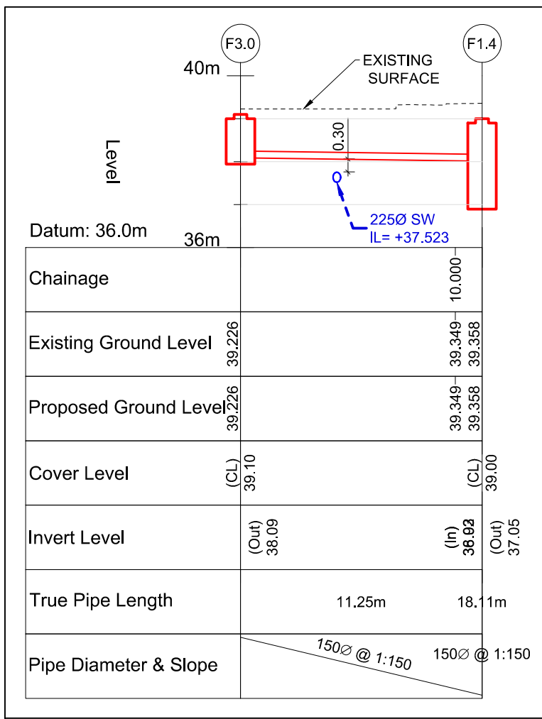
F3 SECTION 1122 SCALE @ A1: H=1:250 ; V=1:125 SCALE @ A3: H=1:500 ; V=1:250
