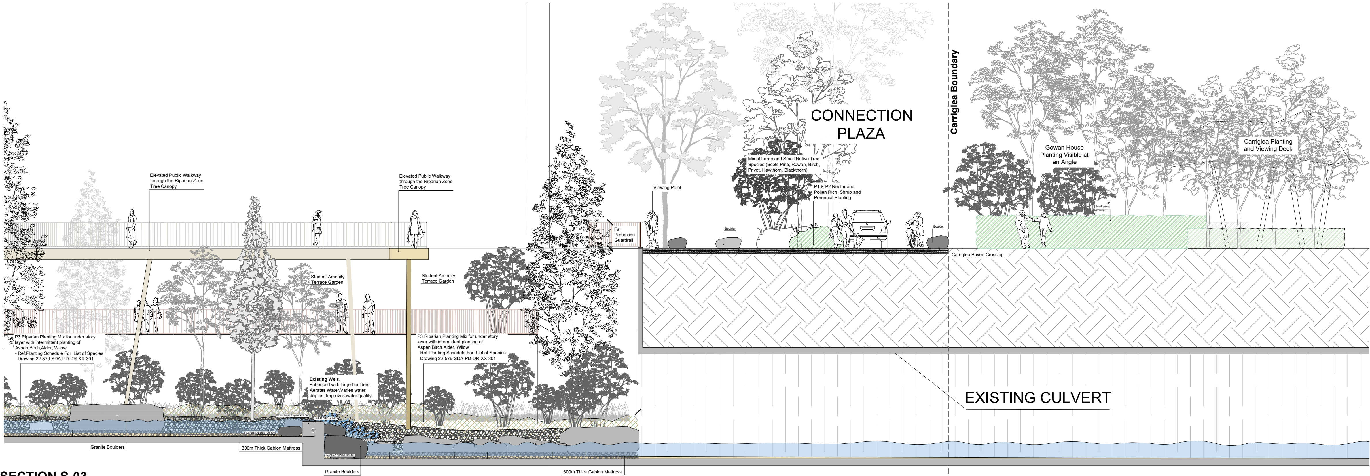
SECTION S-03 Scale 1:100
