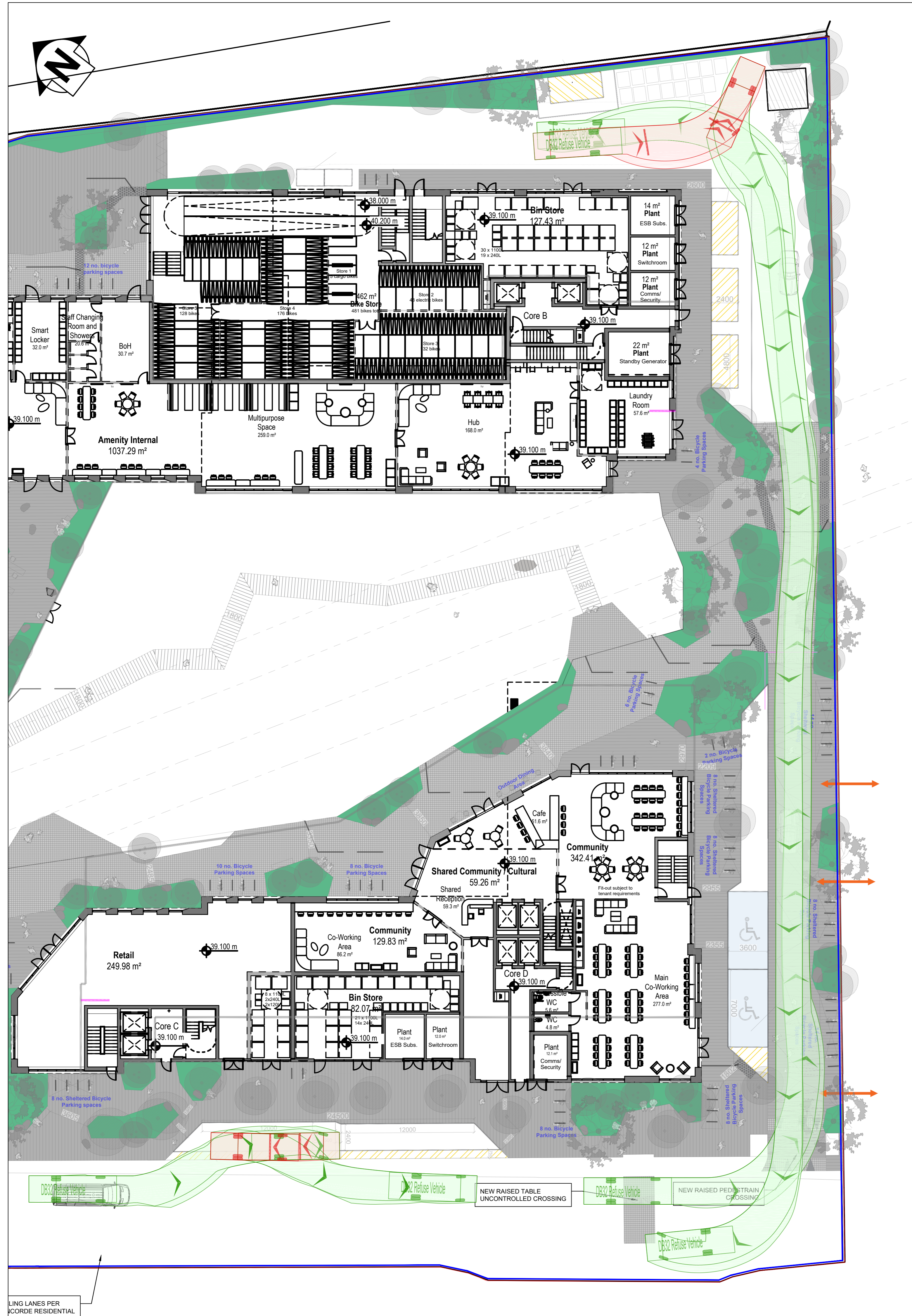
AUTOROUTE TRACKING - REFUSE VEHICLE
