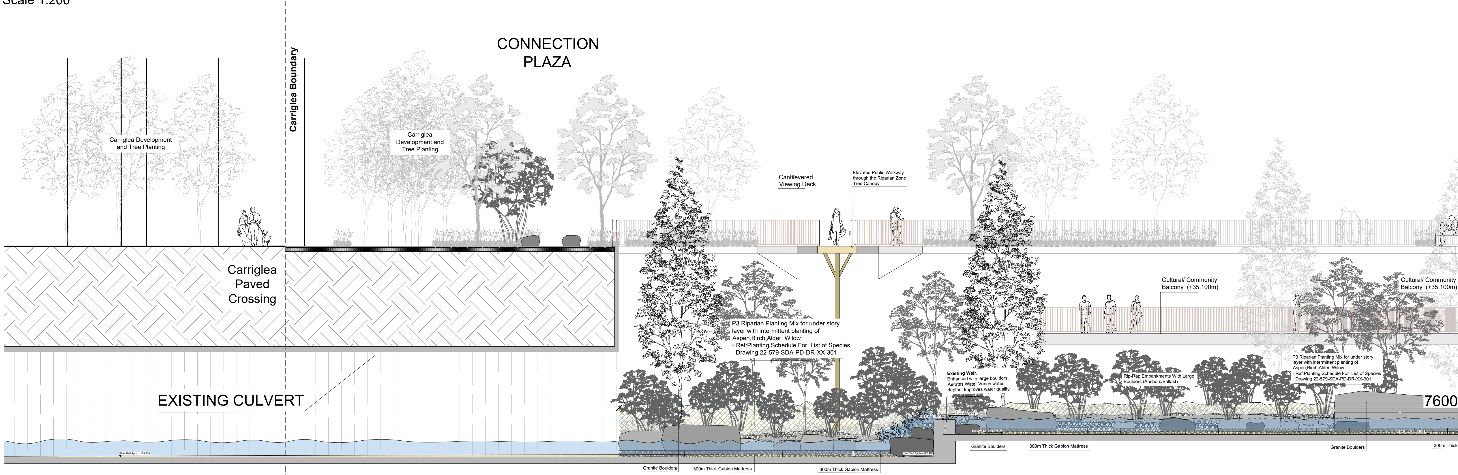
SECTION S-04 Scale 1:100
