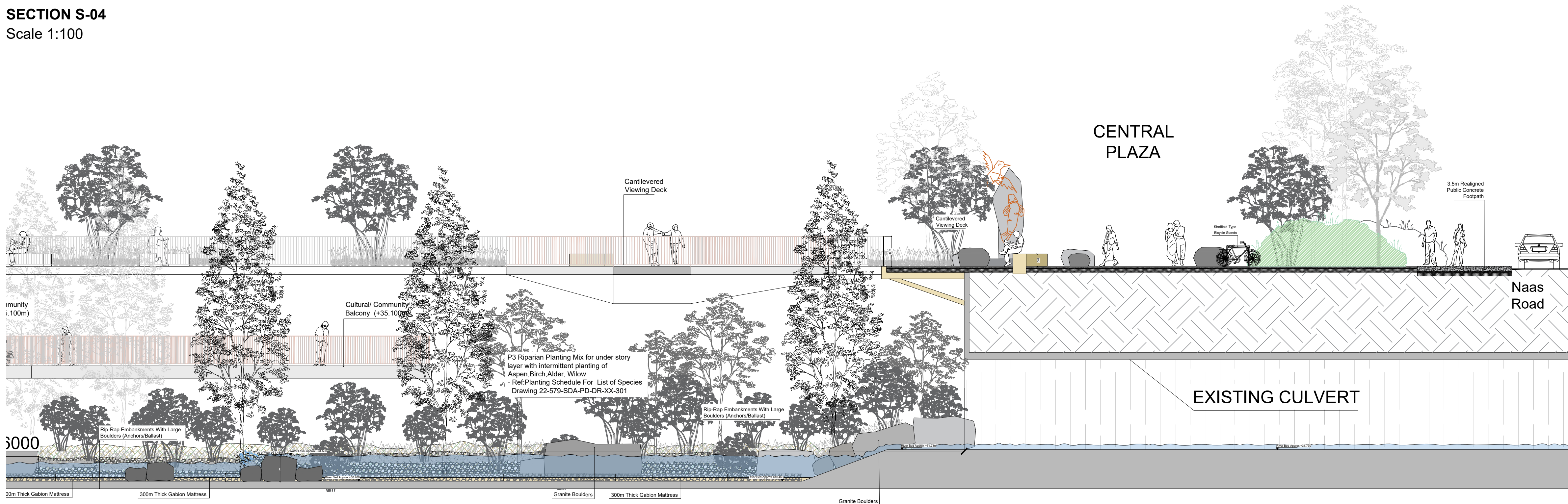
SECTION S-04 Scale 1:100
